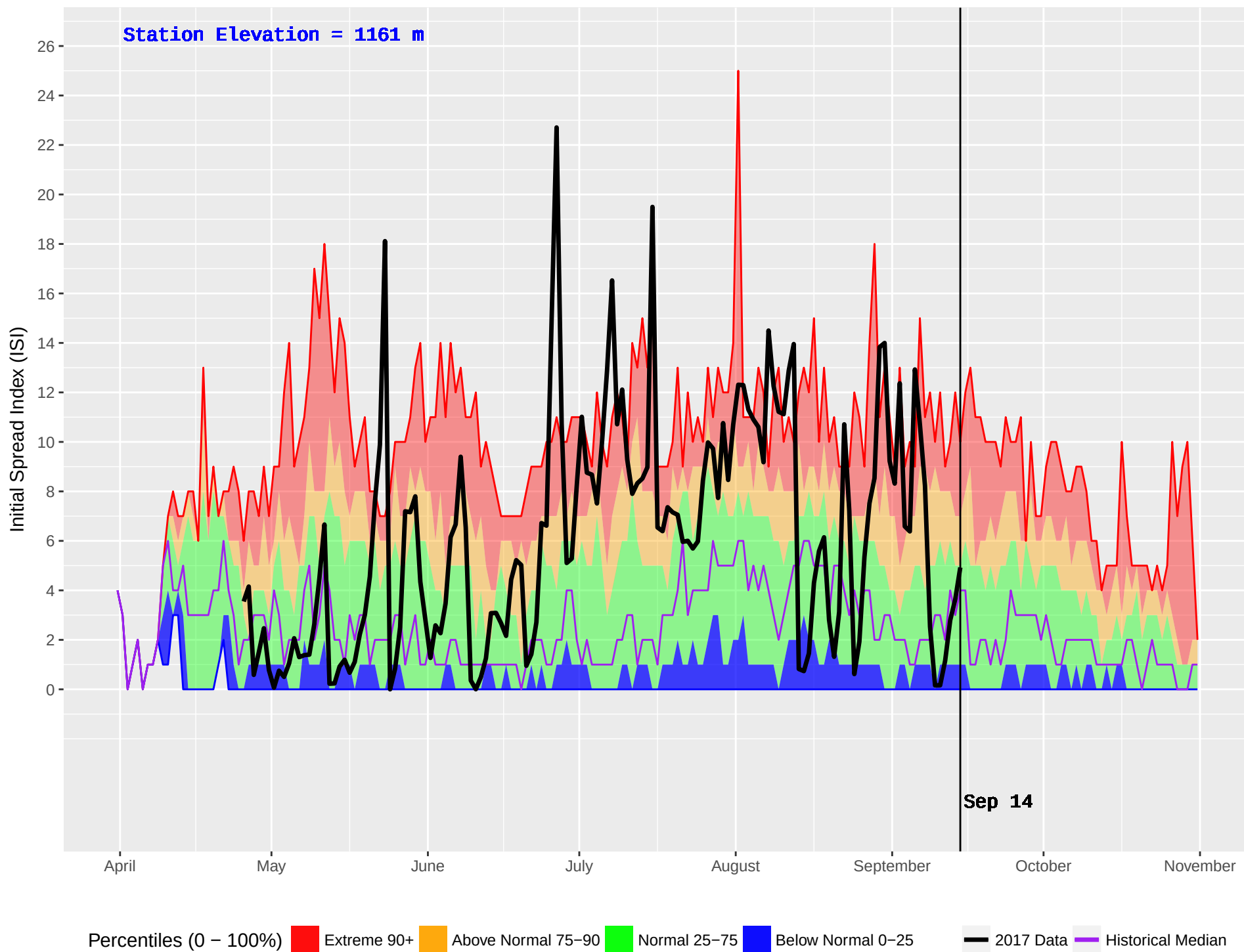
TIMOTHY (234) : Historical (1990–2016) and Current (2017) Noon Initial Spread Index (ISI)
